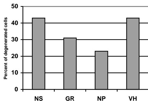
Figure 2. Protective effects of nimodipine and garlic on neuronal degeneration in CA1 hippocampus compared to controls (NS, VH).
